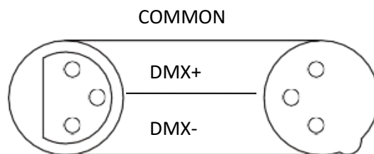
DMX 512 OUT 3-PIN XLR
