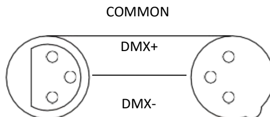
DMX 512 OUT 3-PIN XRL
