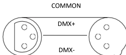
DMX 512 OUT 3-PIN XLR
