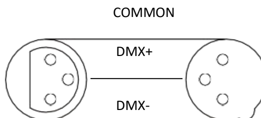
DMX 512 OUT 3-PIN XLR
